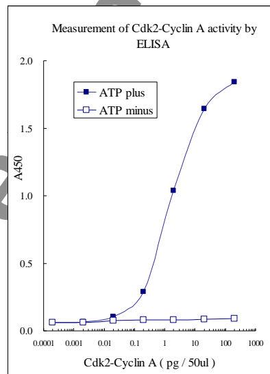
Fig.3 ELISA for measurement of recombinant Cdk2-CyclinA kinase activity using Phospho- Rb Thr356 Monoclonal antibody (4E3)
