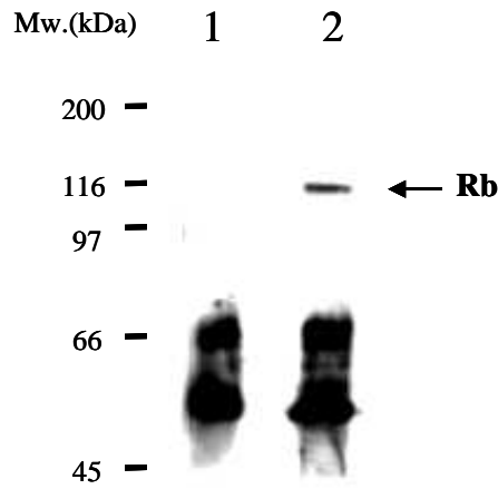
Fig.2 IP-Western blotting phosphorylated Rb using Phospho-Rb Thr356 Monoclonal antibody (4E3)
